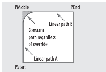
Continuous path function for faster cycle times
