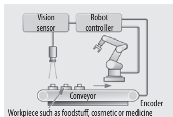
Object tracking function for faster cycle times
